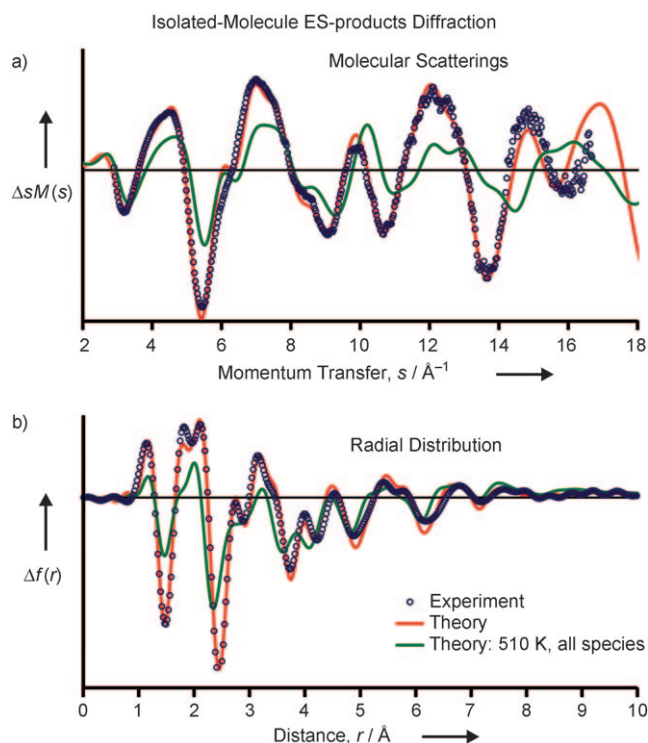
Figure 3. Diffraction results of the excited state (ES)-products structures of 6-nitro-BIPS, following UV excitation. Shown are a) frame-referenced molecular scattering function, \Delta sM(s; t=+100 \text{ ns}, t_{\text{ref}}=-100 \text{ ns}) , and b) the frame-referenced radial distribution, \Delta f(r; t=+100 \text{ ns}, t_{\text{ref}}=-100 \text{ ns}) , for the experimental (circles) and theoretical curves (line). Also shown in green are the difference curves, where all species are held at the temperature of the ground state (510 K), to highlight the contribution due to structural rearrangement.
